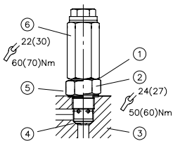
Figure 8: Pressure controlled 2-way directional valve type CNE
