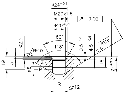
Figure 5: Mounting hole Type CNE 21, CNE 22, CNE 23
