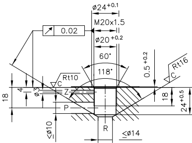
Figure 4: Mounting hole Type CNE 2
