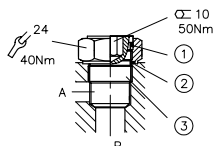
Figure 7: Passage blocked
