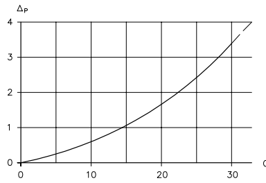
Figure 3: Flow Q (lpm); Flow resistance Δp (bar)
