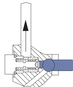
CPRV valve
